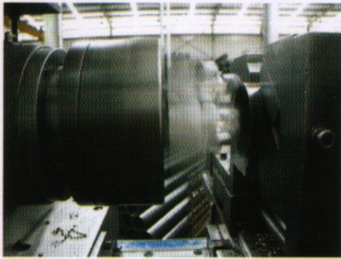
SHELL ENDS ARE MACHINED TO PROVIDE STRAIGHTNESS AND INNER PROFILE FOR PROPER FIT WITH BEARING HOUSING
